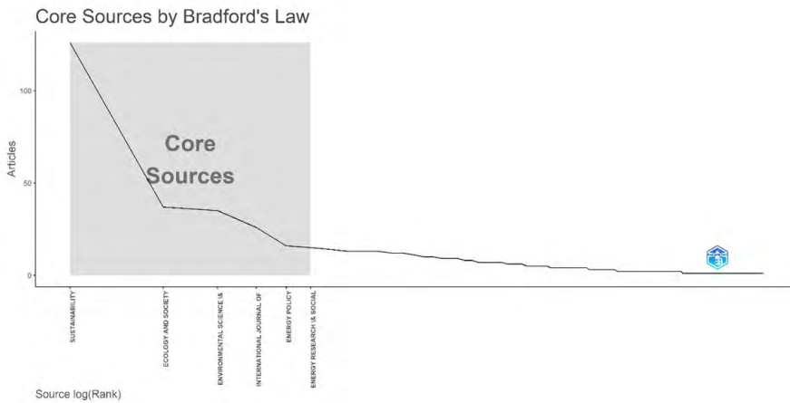
Figura 24. Bradford's Law .
